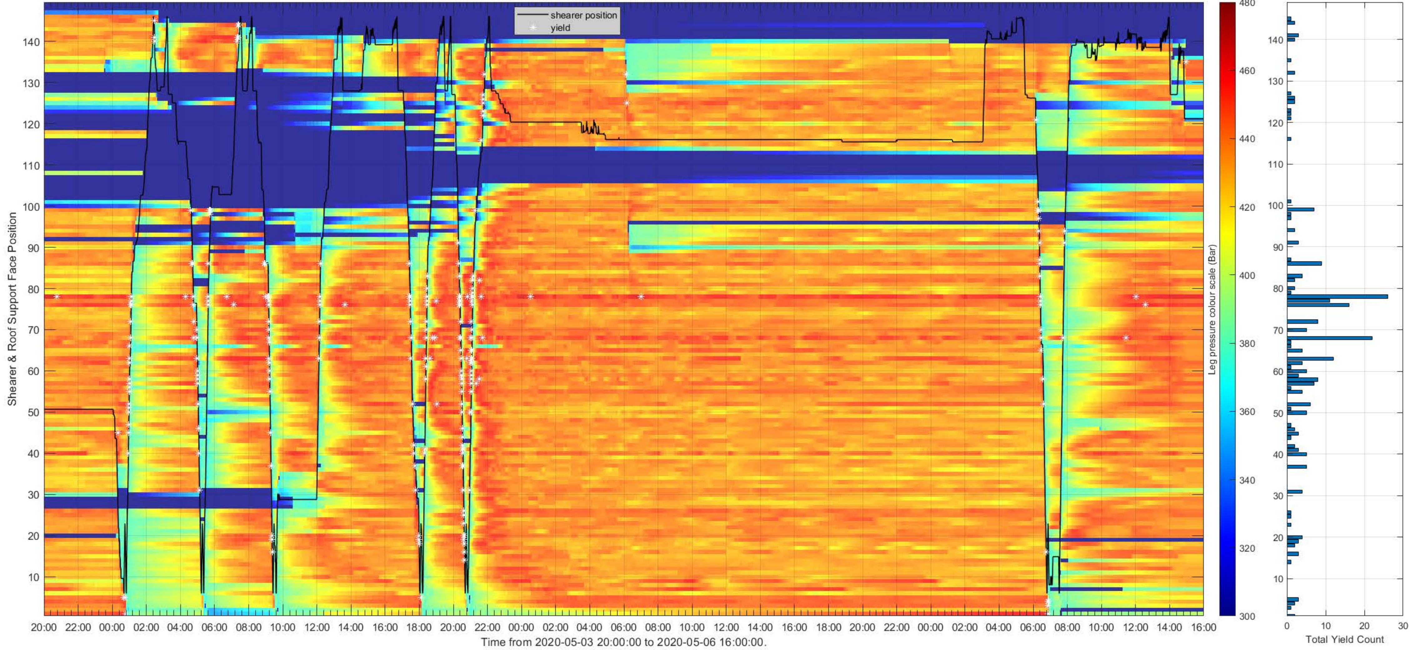
Grosvenor Shearer Position, PRS Leg Pressure (Bar) & Yield Events (*): 2020-05-03 20:00:00 to 2020-05-06 16:00:00.
